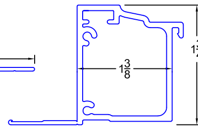
"Traditional" BRICKMOLD(radius)
