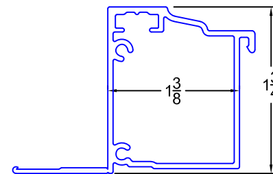
"Traditional" BRICKMOLD
