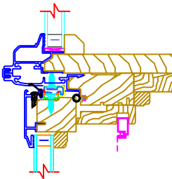
CASEMENT FAMILY FRAME EXPANDERS SHOWN USING 7/8" EXPANDER W/ OPTIONAL 2" AND 3"
