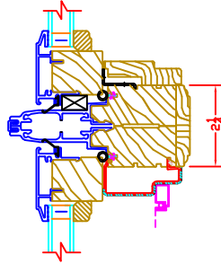
CASEMENT / FIXED CASEMENT AWNING / FIXED CASEMENT 0" Mull Shown W/ OPTIONAL 1', 1 1/2', 2', 3', OR 4'
