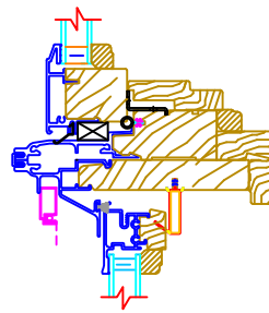
CASEMENT TRANSOM / DOUBLE HUNG 0" Mull Shown W/ OPTIONAL 1', 1 1/2', 2', 3', OR 4'
