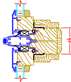
FIXED CASEMENT / FIXED CASEMENT 0" Mull Shown W/ OPTIONAL 1', 1 1/2', 2', 3', OR 4'
