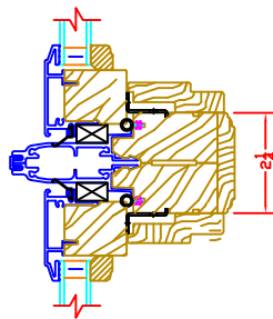
CASEMENT TRANSOM / FIXED CASEMENT 0" Mull Shown W/ OPTIONAL 1', 1 1/2', 2', 3', OR 4'
