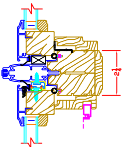
CASEMENT TRANSOM / CASEMENT CASEMENT TRANSOM / AWNING 0" Mull Shown W/ OPTIONAL 1', 1 1/2', 2', 3', OR 4'
