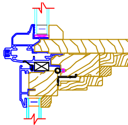
RADIUS / FIXED CASEMENT 0" Mull Shown W/ OPTIONAL 1', 1 1/2', 2', 3', OR 4'
