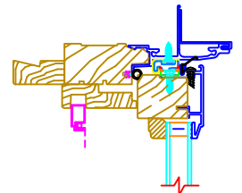
CASEMENT FAMILY DRIP CAP APPLICATION
