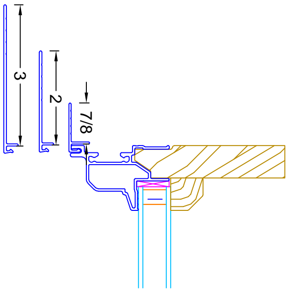
USA REPLACEMENT FIXED LITE FRAME EXPANDERS SHOWN USING \frac{7}{8} EXPANDER W/ OPTIONAL 2" AND 3"
