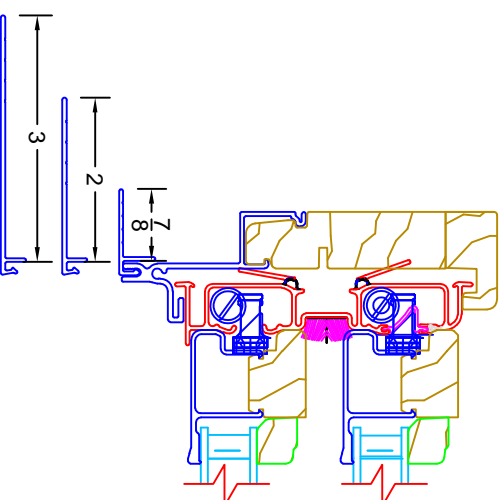
DOUBLE HUNG FAMILY FRAME EXPANDERS SHOWN USING 7/8" EXPANDER W/ OPTIONAL 2" AND 3" EXPANDERS
